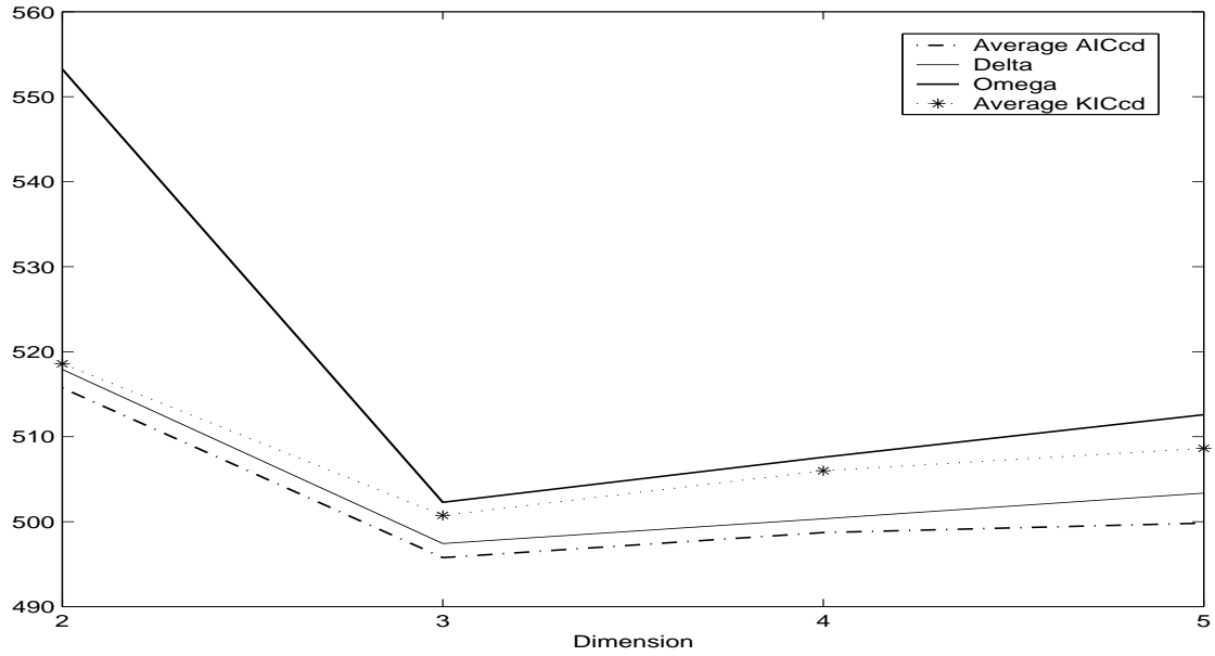
Figure 1. \Omega_{\mathbf{Y}}(d, \theta_0) , \Delta_{\mathbf{Y}}(d, \theta_0) and Average values of KICcd and AICcd curves (bivariate normal simulation set 3)
