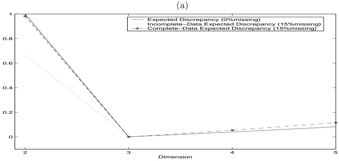
Figure 2. Simulated \Omega_{\mathbf{Y}}(d, \theta_0) and \Omega_{\mathbf{Y}_o}(d, \theta_0) curves for bivariate normal simulation.
