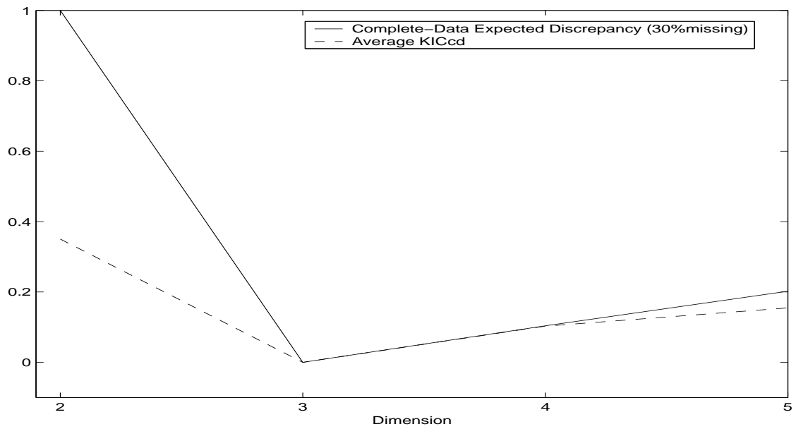
Figure 3. Simulated \Omega_{\mathbf{Y}}(d, \theta_0) and Average KICcd curves (bivariate normal simulation set 3)
